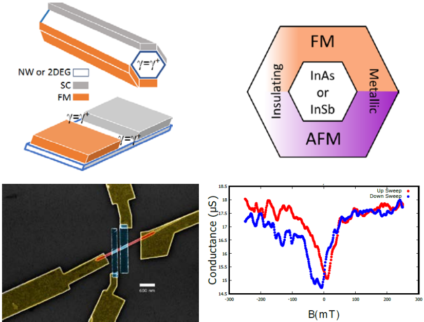
Fig. 1: (top-left) Schematic of devices integrating a ferromagnet (FM), semiconductor and superconductor (SC) for realizing Majorana zero modes. We will explore both 1D platforms based on semiconductor nanowires (NW) (top) and platforms based on two-dimensional electron gases (2DEG) (bottom). (top-right) Conceptual representation of materials phase space to be considered for magnetic materials coupled to InAs and InSb nanowires. (bottom) Example of a device consisting of an InSb nanowire with FM and normal contacts, and measured hysteretic resistance from a similar device.
