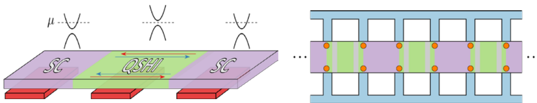
Left: A setup for realizing 4\pi -periodic Josephson effect with a junction in a single flake of WTe_2 with electron density controlled with gates below to allow tuning between SC and QSHI regimes. Right: A quantum information processing architecture based on a monolayer of WTe_2 with periodic arrangement of SC (violet) and QSHI (green) regions. Blue leads are normal metal with a long phase coherence length, which can be gated to form loops connecting different Majorana states across the system. Measuring the current in the loop will enable projective measurements of Majorana bilinears.
