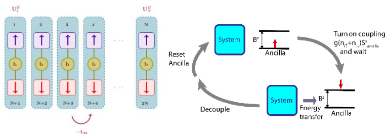
Fig. 1: Cooling algorithm to be employed in describing driven-dissipative systems on near-term quantum computers for project one.
